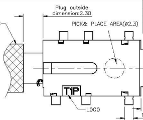
( \phi 3.50\text{mm} 4 POLE PLUG DETAIL DRAWING)
