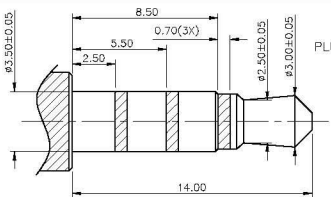
( \phi 3.50\text{mm} 4 POLE PLUG DETAIL DRAWING)
