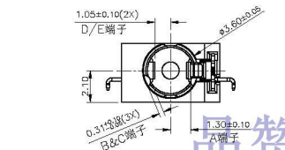
( \phi 3.50\text{mm} 4 POLE PLUG DETAIL DRAWING)
