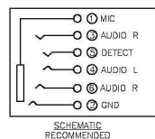
SCHEMATIC RECOMMENDED
