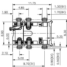
RECOMMENDED PCB LAYOUT TOP VIEW T=0.50mm,TOL:±0.05
