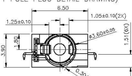
(Ø3.50mm 4 POLE PLUG DETAIL DRAWING)
