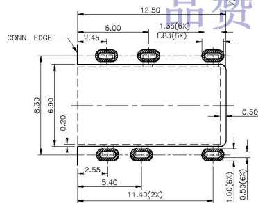
RECOMMENDED PCB LAYOUT (COMPONENT SIDE) T=0.60mm, TOL:±0.05
