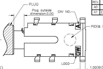
(ø3.50mm 4 POLE PLUG DETAIL DRAWING)
