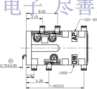
SCHEMATIC RECOMMENDED
