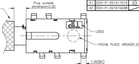
(Ø3.50mm 4 POLE PLUG DETAIL DRAWING)
