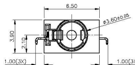
(Ø3.50mm 4 POLE PLUG DETAIL DRAWING)
