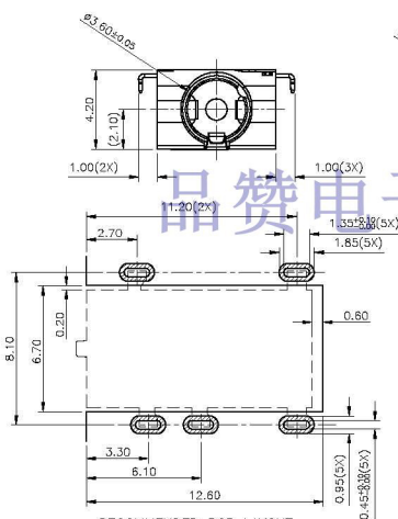
RECOMMENDED PCB LAYOUT TOP VIEW TOL:±0.05
