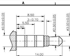
(ø3.50mm 4 POLE PLUG DETAIL DRAWING)
