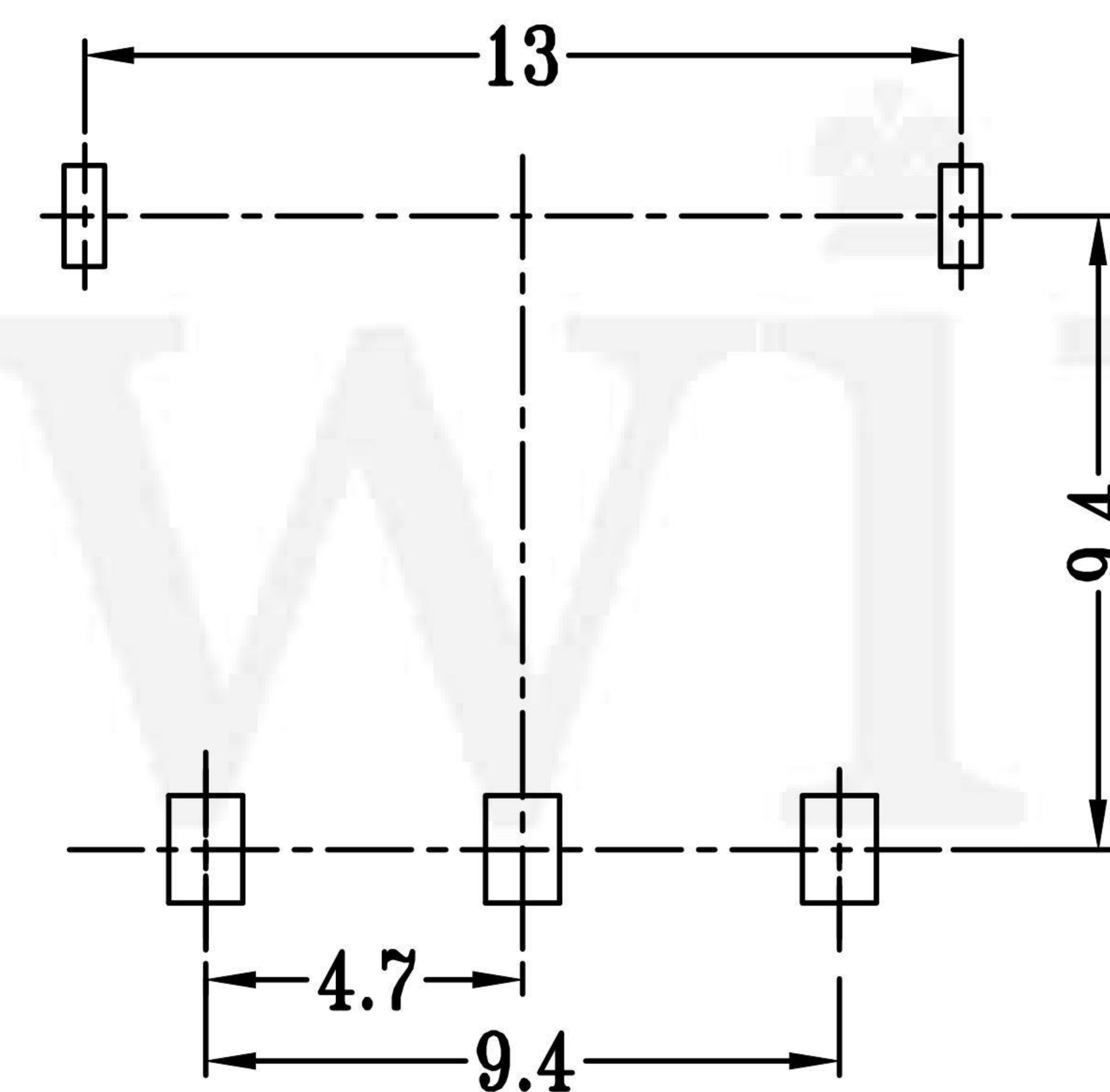
P.C.B LAYOUT BOTTOM VIEW
