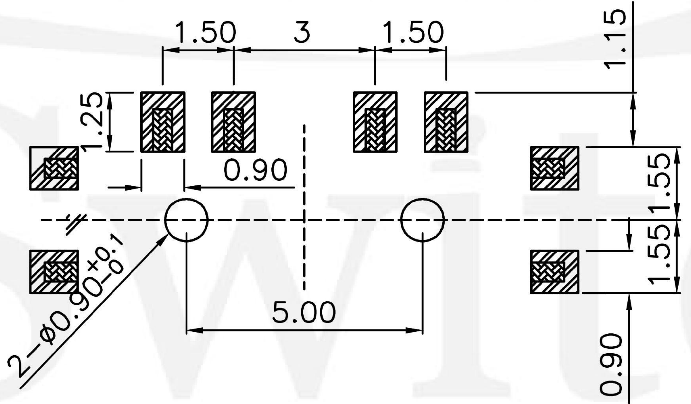
PCB PLERTING PLAN
