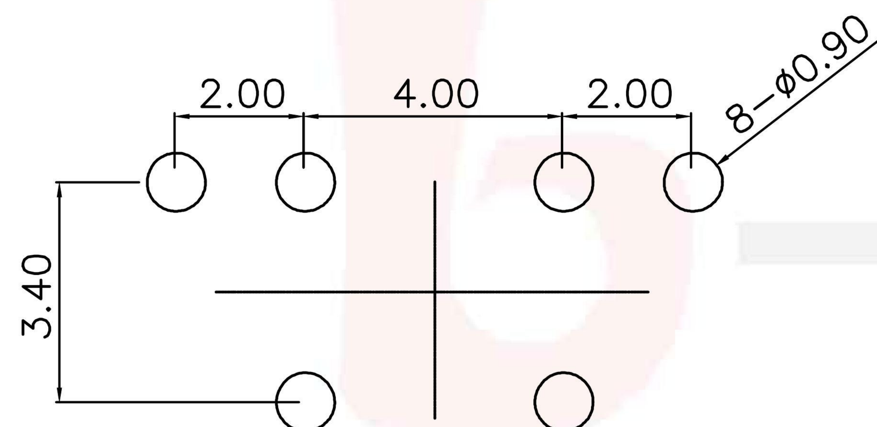
PCB LAYOUT PLAN
