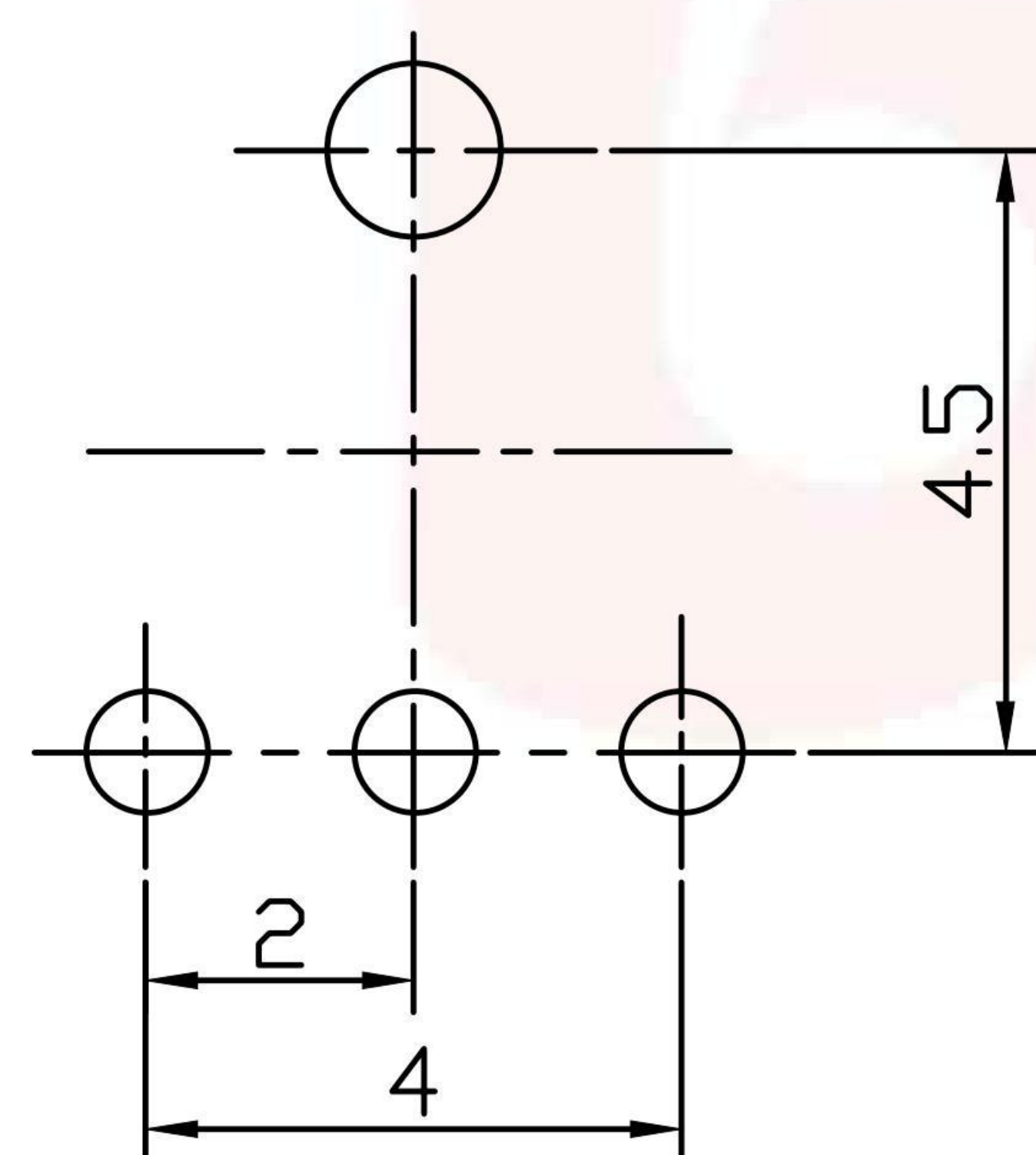
P.C.B LAYOUT BOTTOM VIEW
