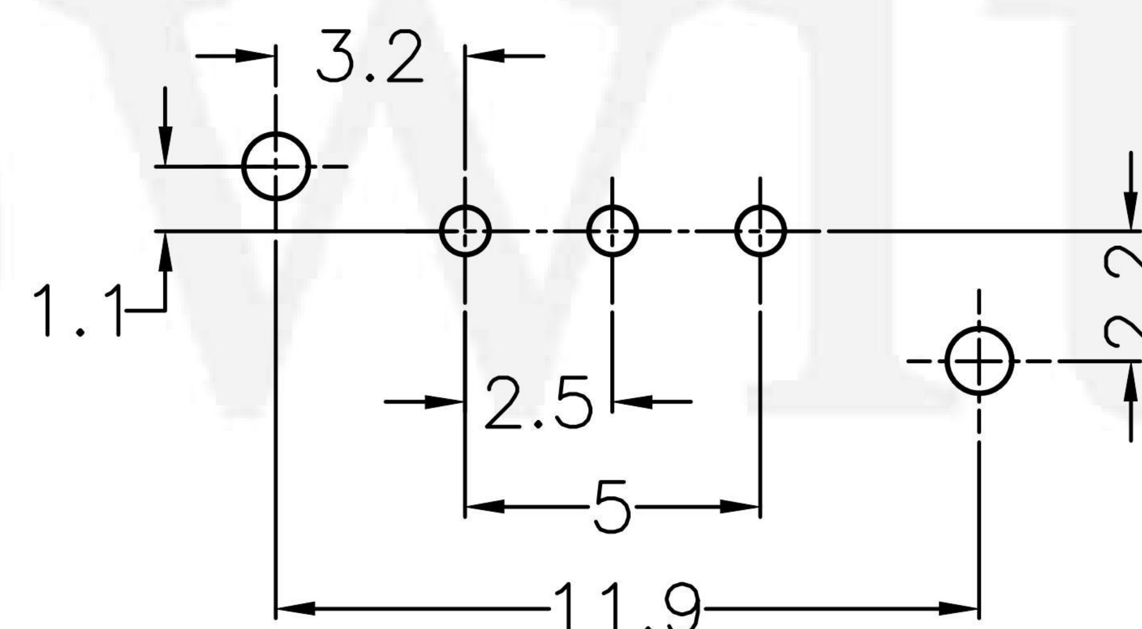
P.C.B LAYOUT BOTTOM VIEW
