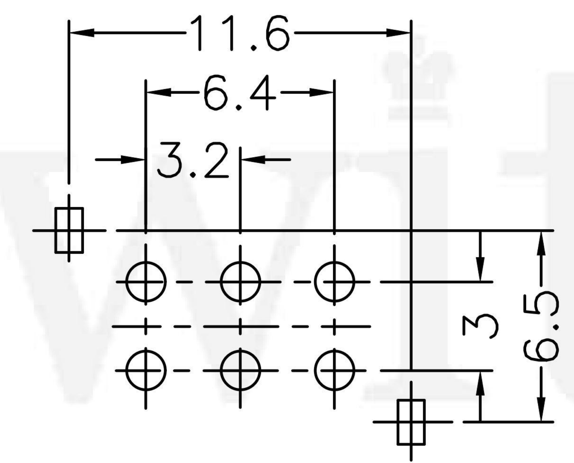
P.C.B LAYOUT BOTTOM VIEW
