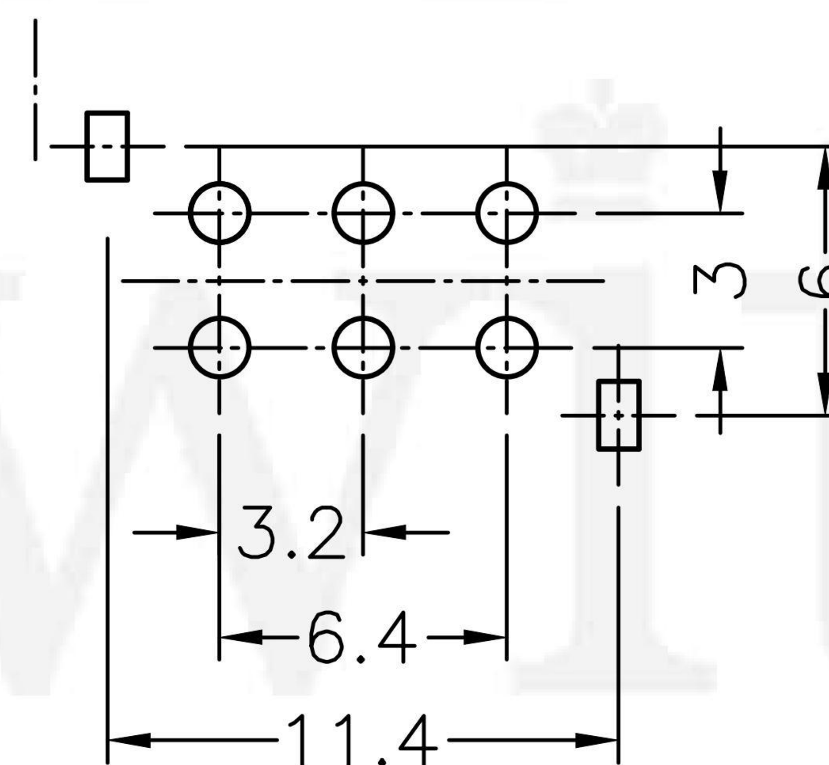
P.C.B LAYOUT BOTTOM VIEW
