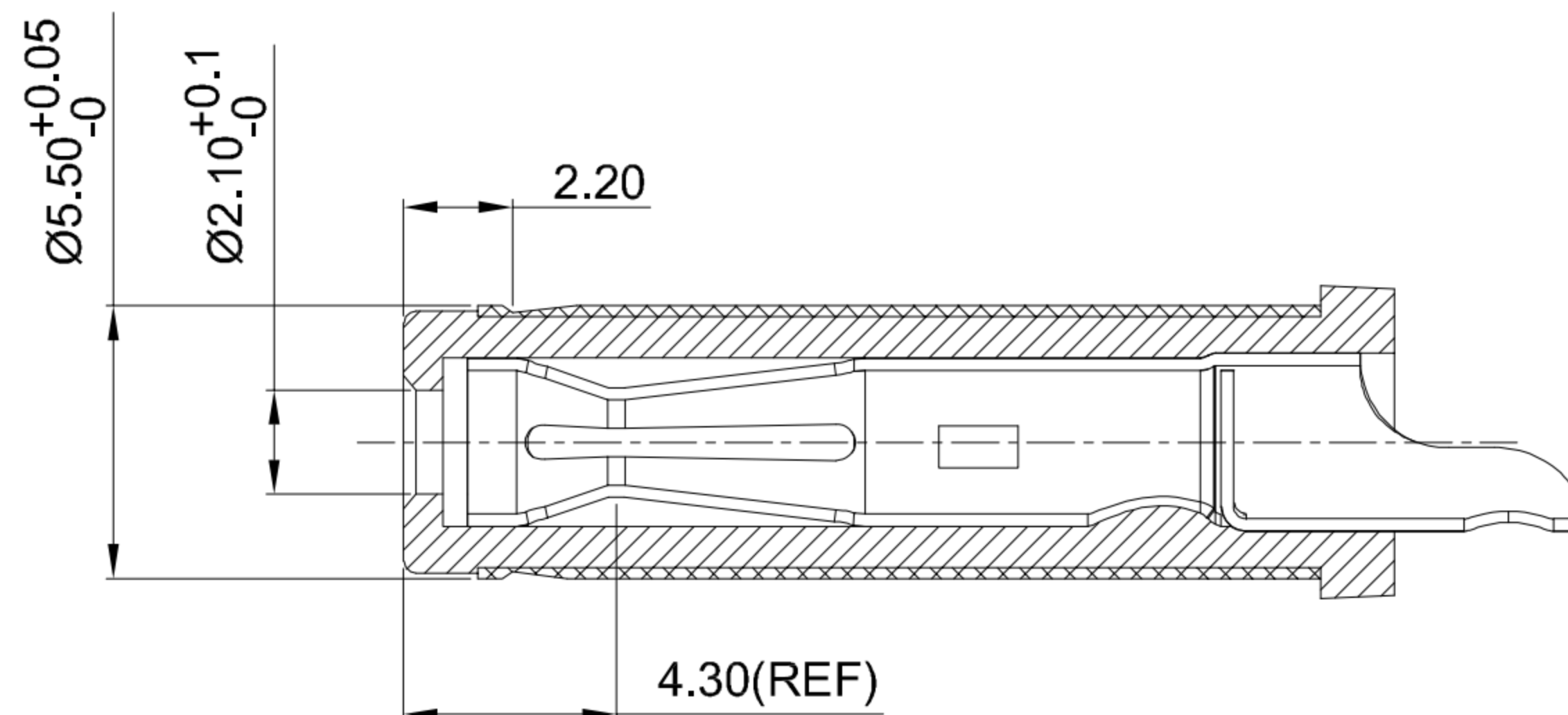
MATING PLUG Ø5.5xØ2.1mm
