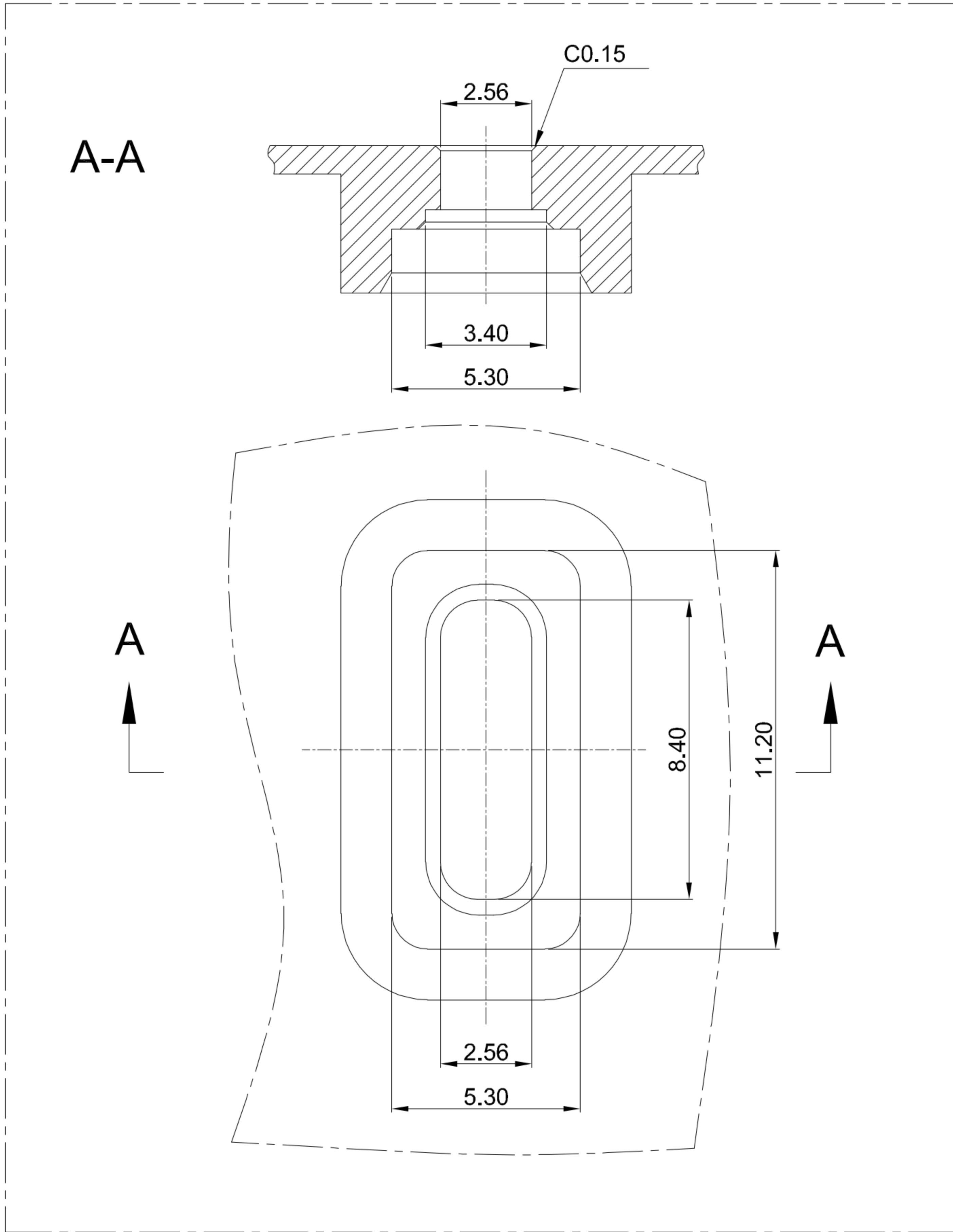
Shell Reference Design Drawing
