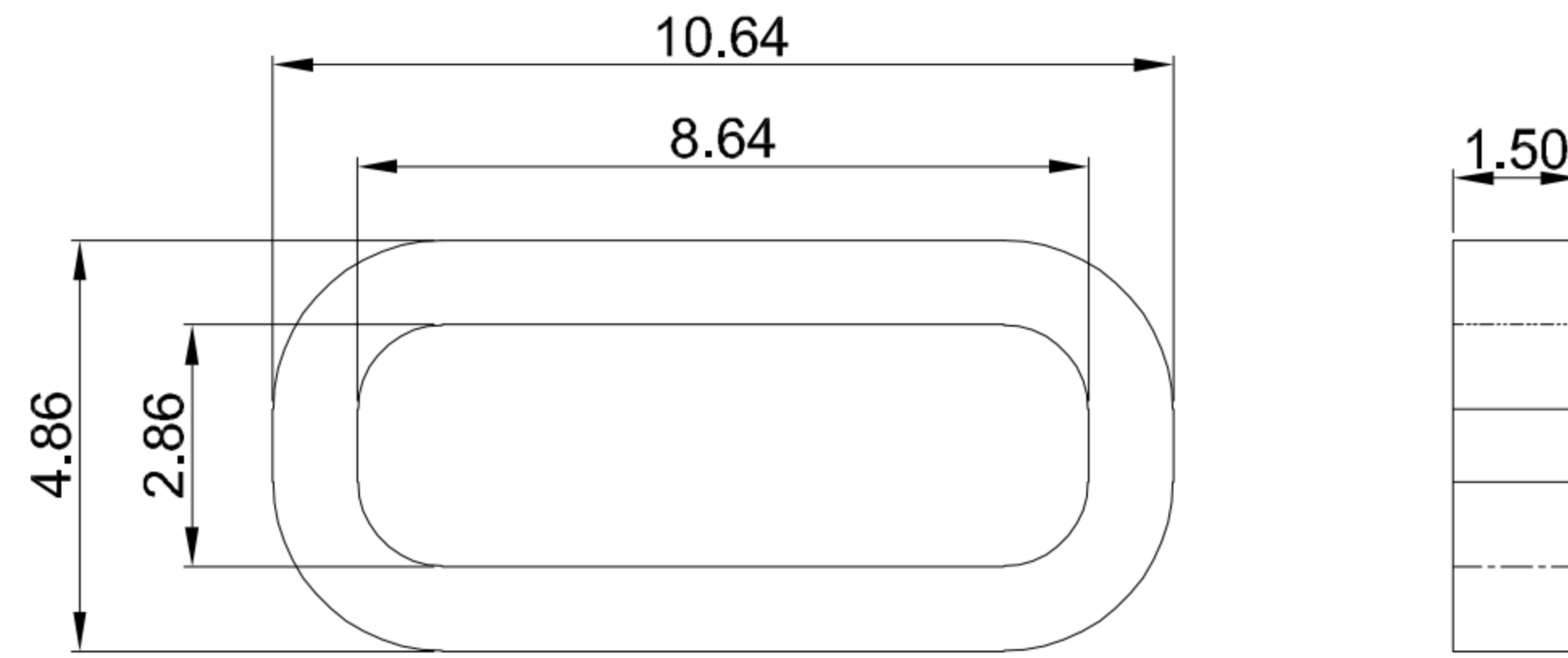
SUGGESTED RUBBER RING SIZE
