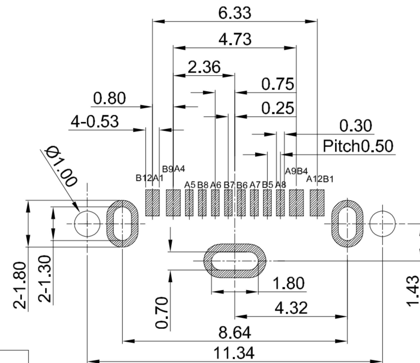
RECOMMENDED PCB LAYOUT TOLERANCE:±0.05
