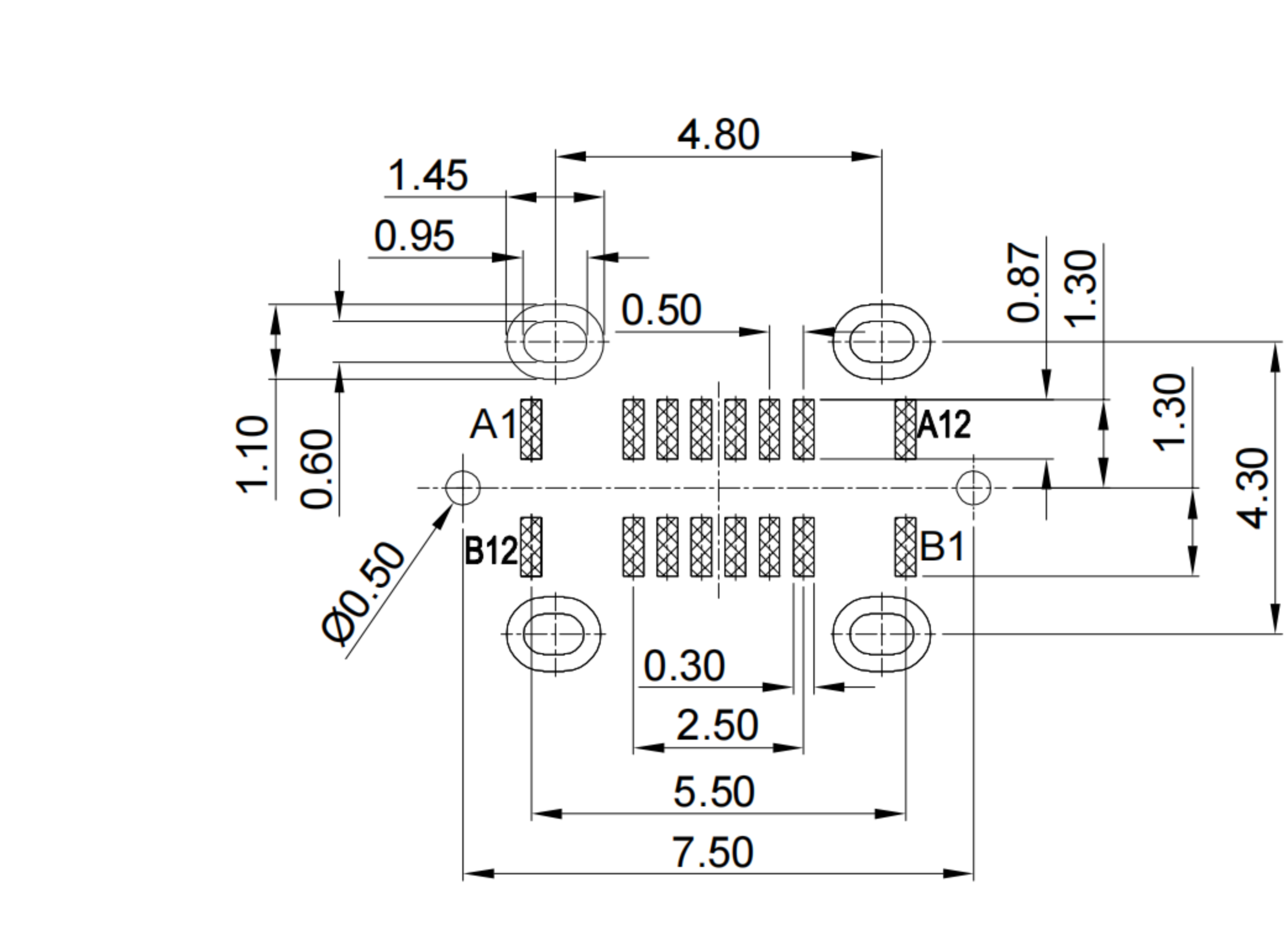
RECOMMENDED PCB LAYOUT TOLERANCE: ±0.05
