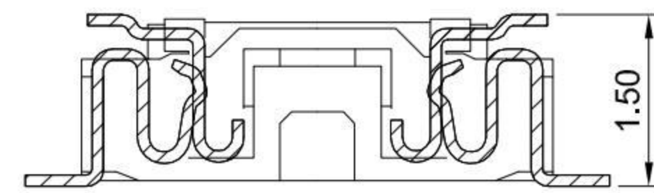
MATING HEIGHT
