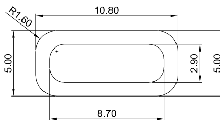
SUGGESTED RUBBER RING SIZE
