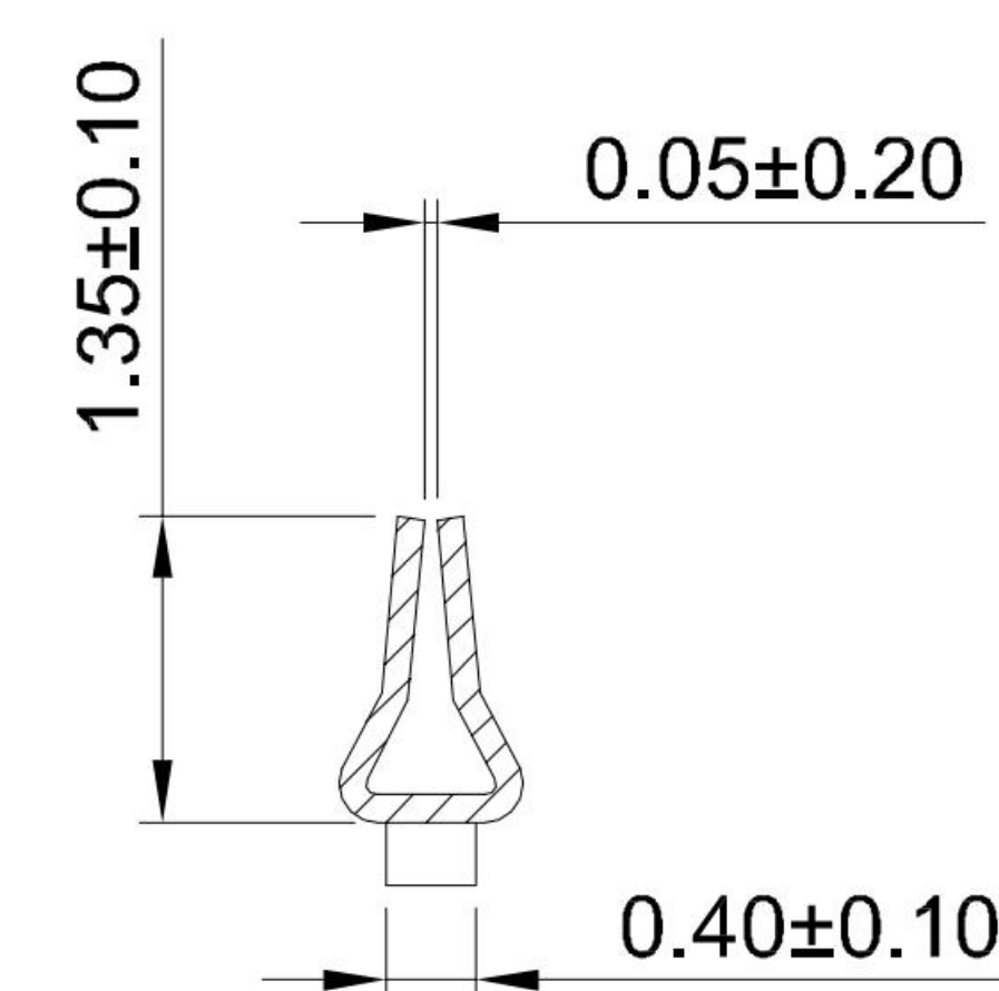
SECTION:C-C
