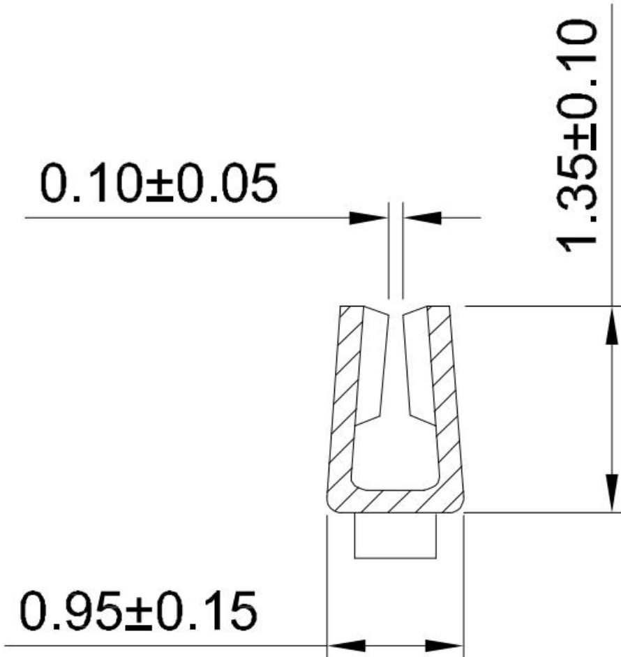
SECTION:C-C
