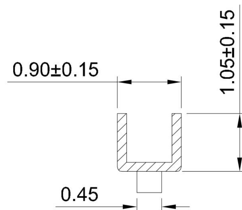
SECTION:C-C
