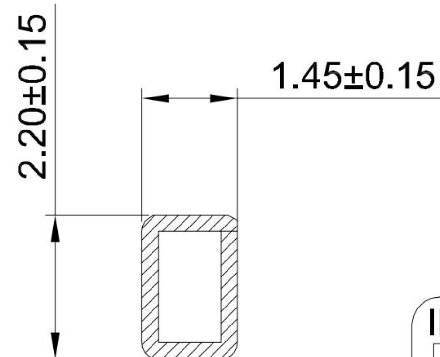
SECTION:C-C
