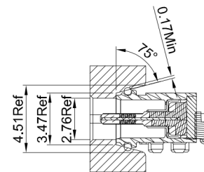
CASE ASSEMBLY FOR REFERENCE
