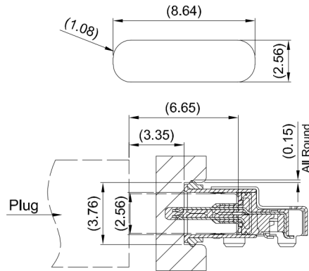
AFTER MATING
