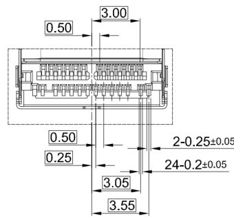
DETAIL OF C
