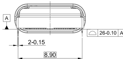
AFTER MATING
