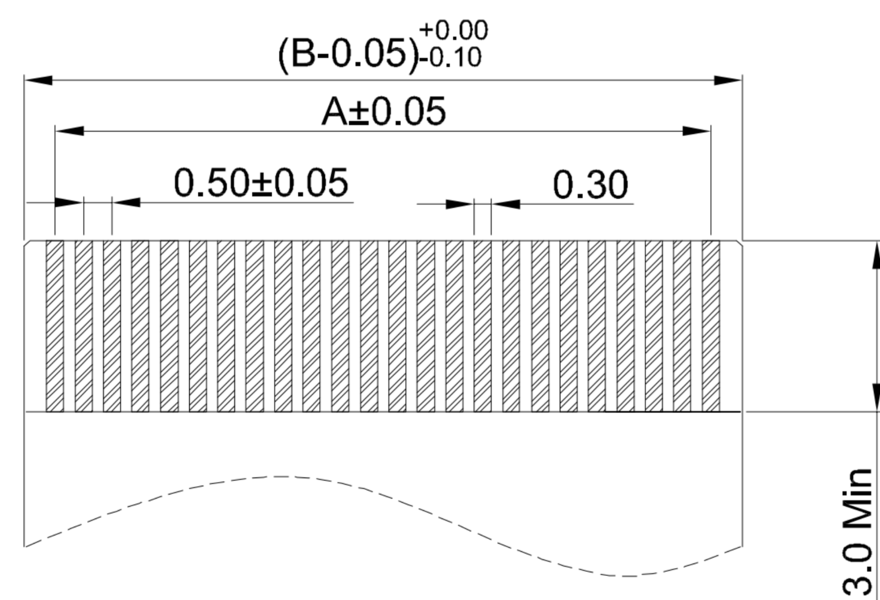
APPLICABLE FPC
