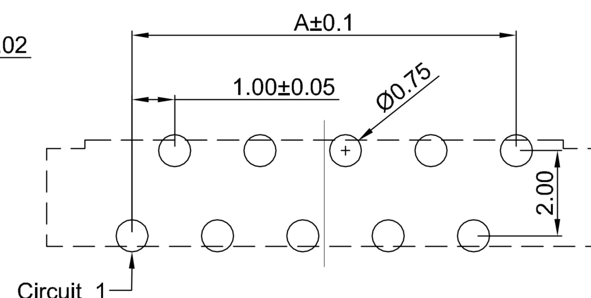
RECOMMENDED PCB LAYOUT TOLERANCE:±0.05
