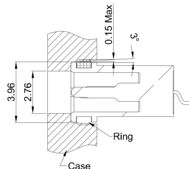
REFERENCE ASSEMBLY
