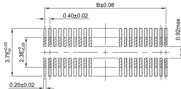
PCB REFERENCE DIAGRAM TOLERANCE:±0.05
