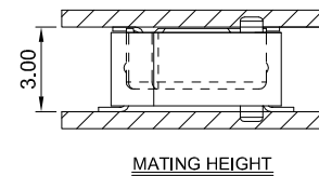
MATING HEIGHT
